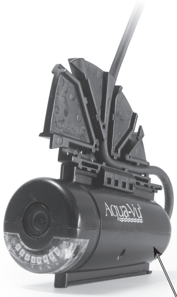
Color Camera with 100' of Cable Featuring All NEW XD Camera Housing™ with Adjustable Quick Attachment Fin System
